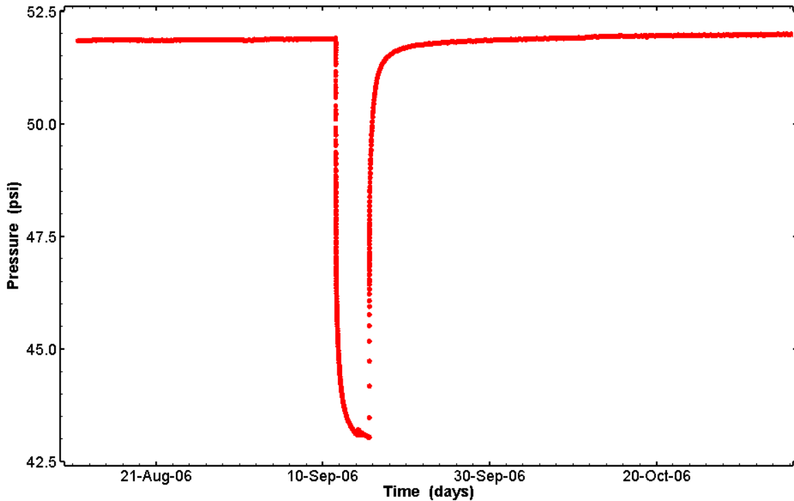
Figure 26. Pressure data from SNL-17A.
