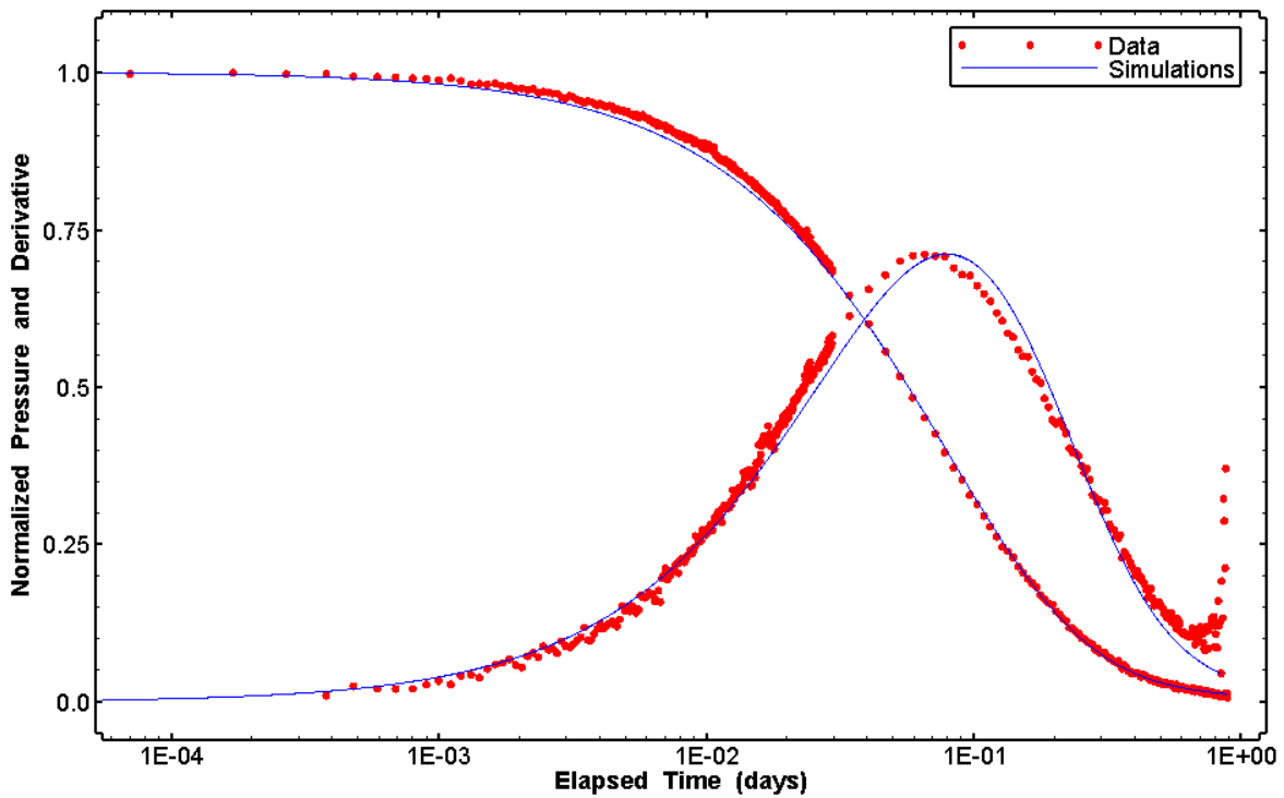
Figure 8. Semilog plot showing 495 simulations of the SNL-8 Ramey A and derivative response.
