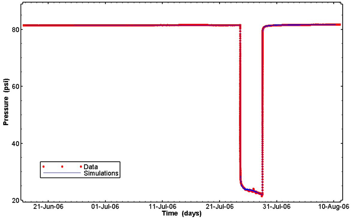
Figure 39. Linear plot showing 239 simulations of the SNL-19 pressure response.
