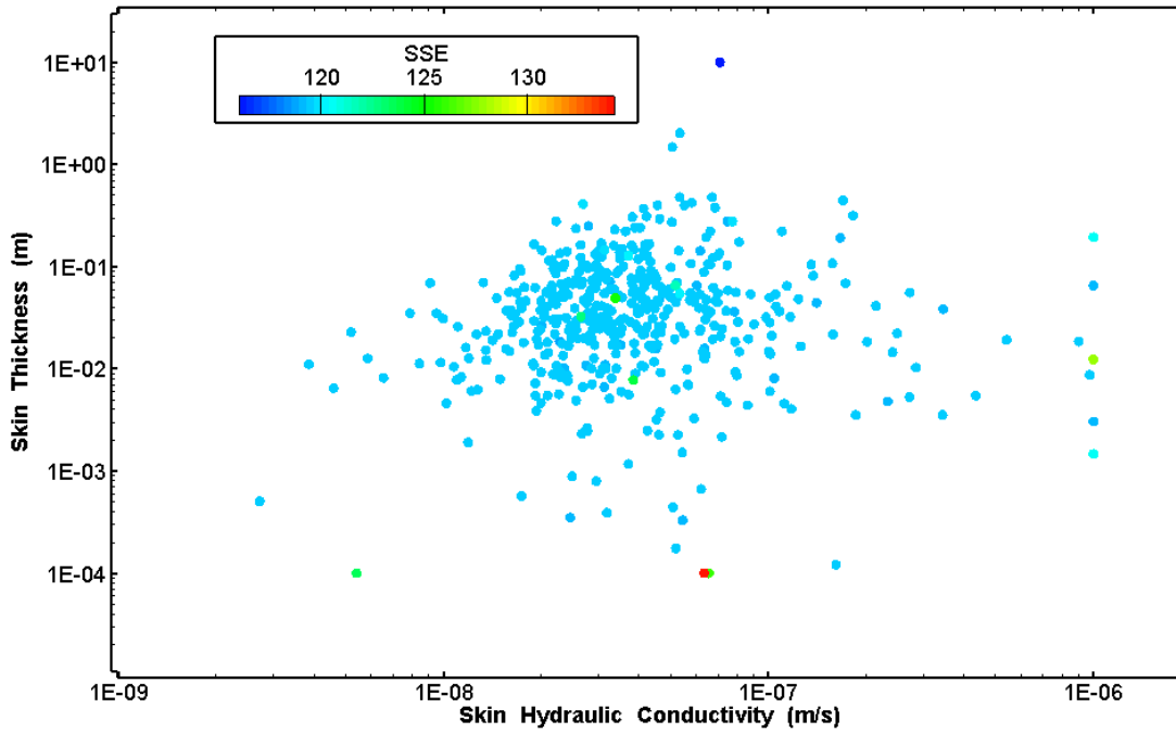
Figure B-3. Estimates of skin hydraulic conductivity and thickness derived from the SNL-10 perturbation analysis.
