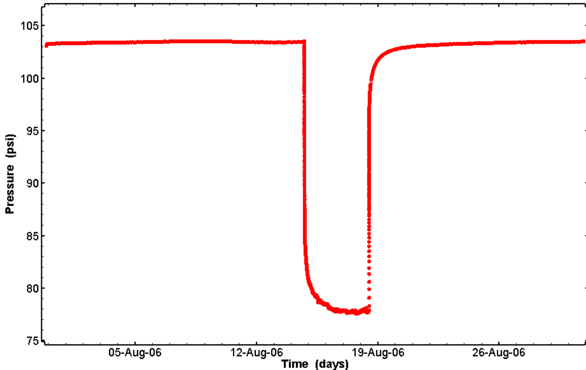
Figure 31. Pressure data from SNL-18.
