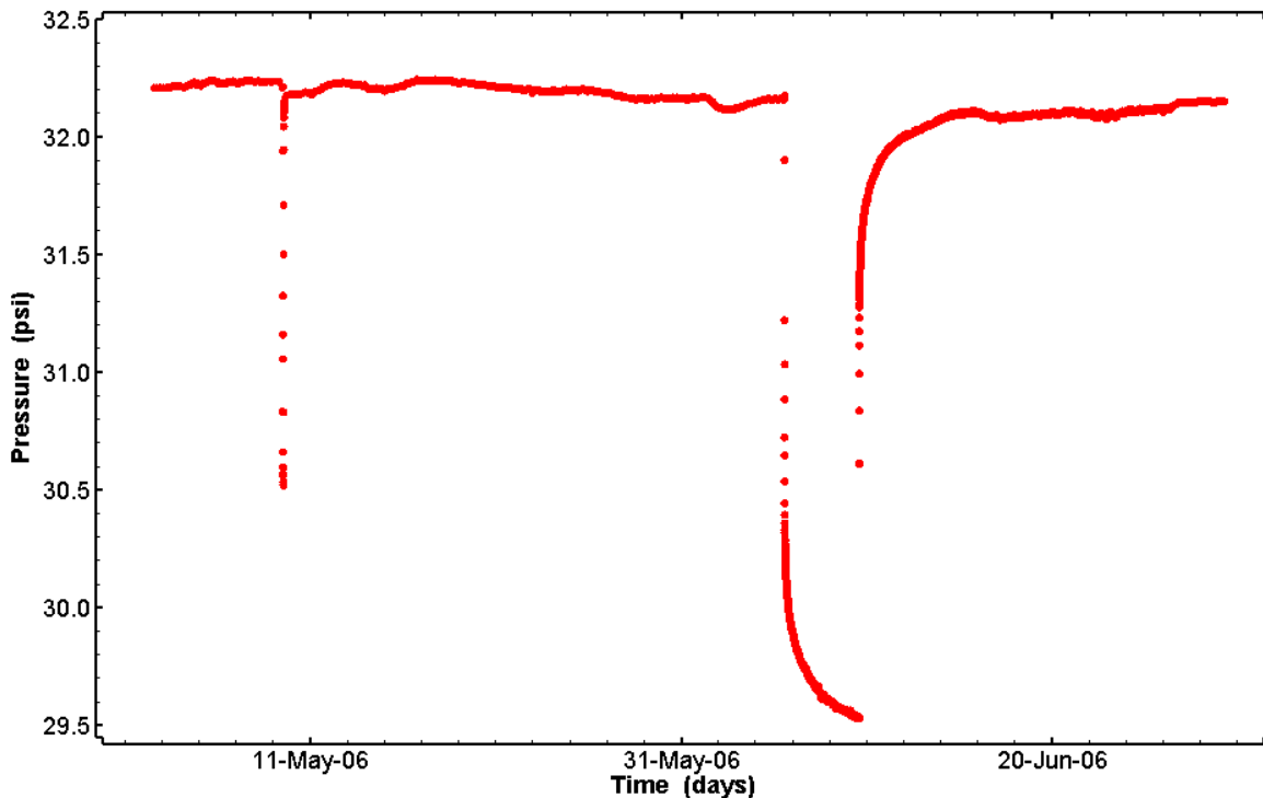
Figure 21. Pressure data from SNL-16.
